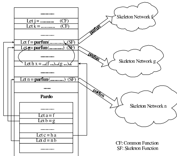
Figure 2: Parallel execution model: the role of parfun and pardo skeleton
